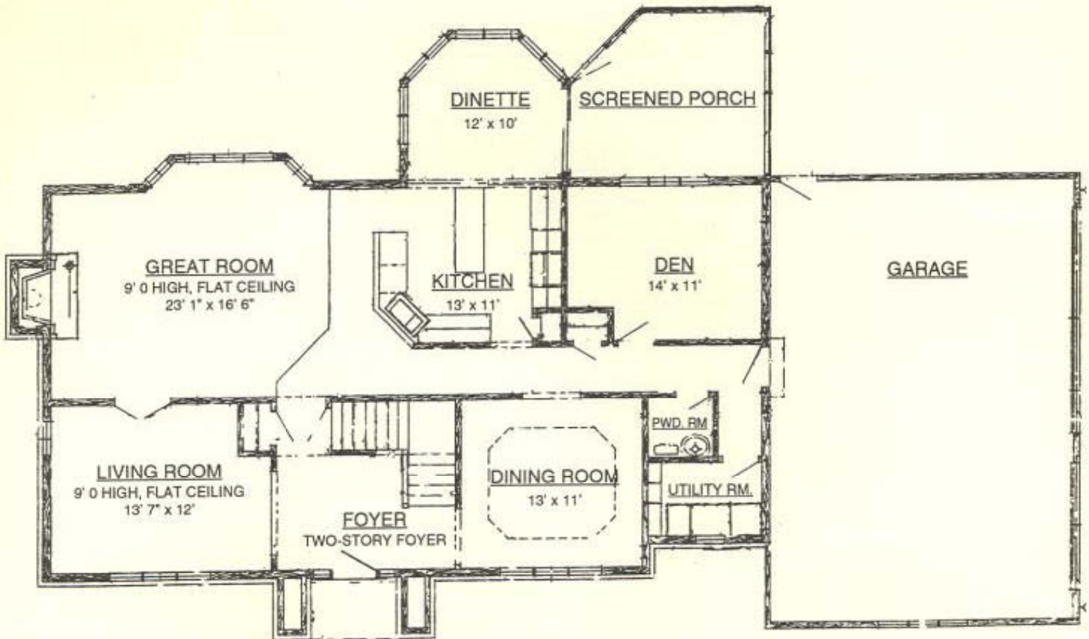
FIRST FLOOR PLAN 1584 Sq. Ft.
