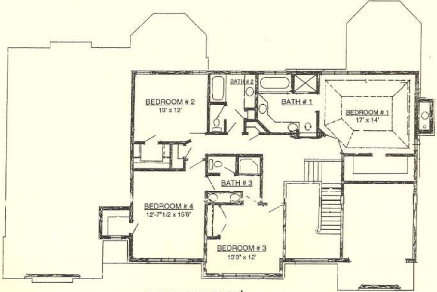
2ND FLOOR PLAN 1459 sq. ft.
